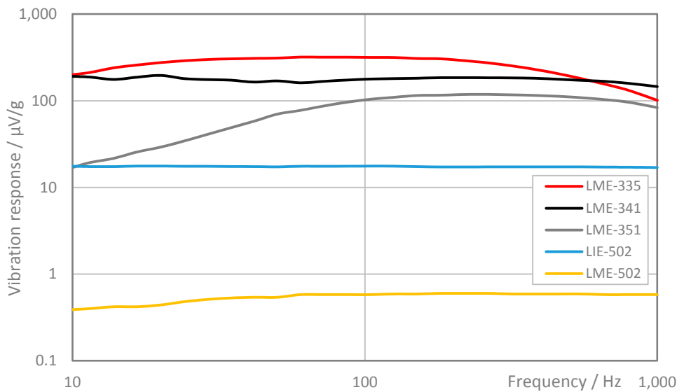
Figure 30: Measurement results of the vibration response across the mechanical excitation frequency: LME-335 (CM, (2 \times 2) mm 2 , 'low micro', 100 G \Omega || 0,2 pF), LME-341 (CM, (2 \times 2) mm 2 , 'low micro', 24 G \Omega || 0.2 pF), LME-351 (CM, (2 \times 2) mm 2 , 'low micro', 5 G \Omega || 0.2 pF), LIE-502 (VM, (3 \times 3) mm 2 , conventional), LME-502 (VM, (3 \times 3) mm 2 , 'low micro')
